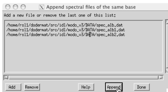
Figure 4.24: The input file list widget 'Append spectral files of the same base'.
