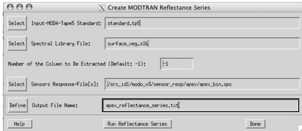
Figure 4.20: The input widget for MODTRAN ® -5 reflectance series.
