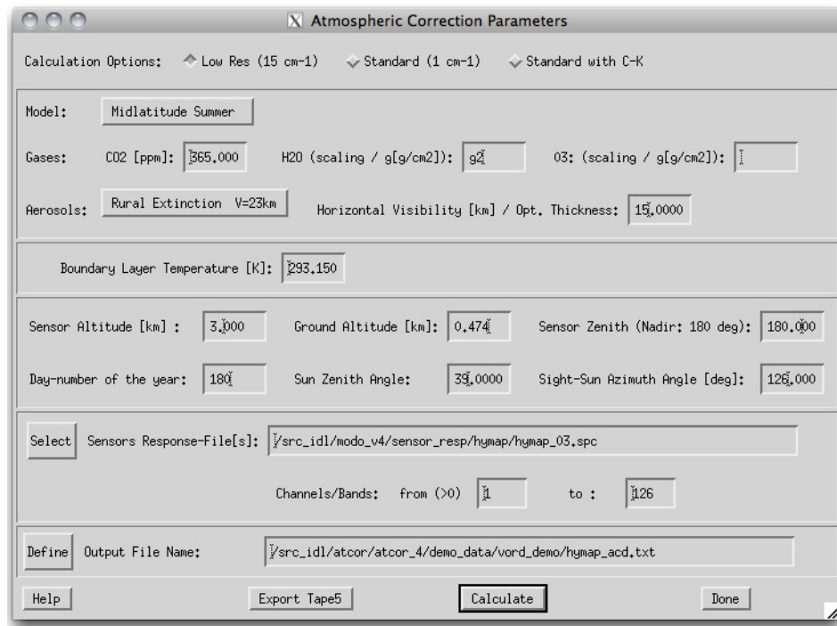
Figure 4.18: Preparation of atmospheric correction parameters.
