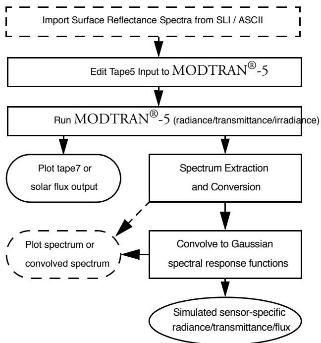
Figure 3.1: Typical workflow structure used for the simulation of imaging spectrometer data.
